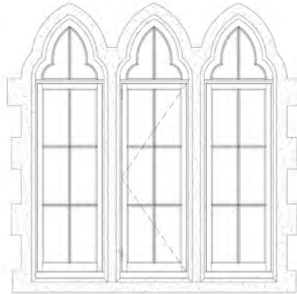
WG 01 Left side elevation View from outside
