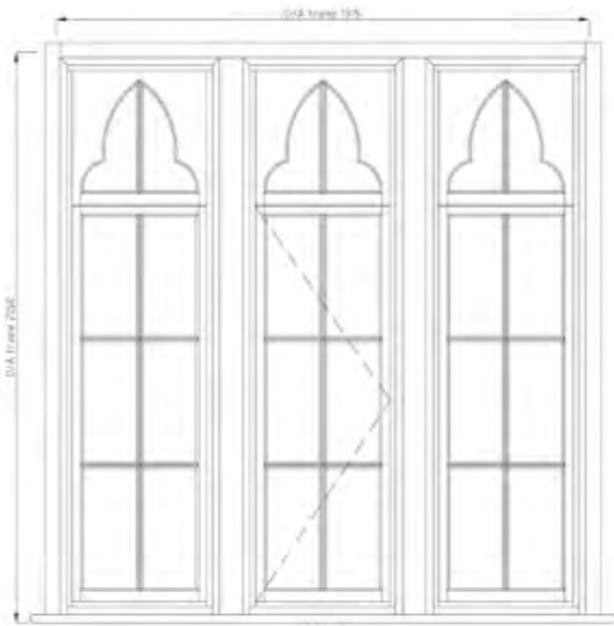
WG 01 Left side elevation View from inside
